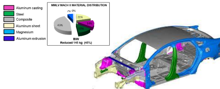
Figure 1.2. Multi Material Lightweight Vehicles MMLV [13]
